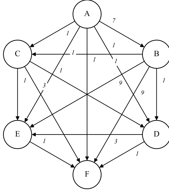
Fig. 4: B-IMDC-u counterexample on an acyclic tournament graph
