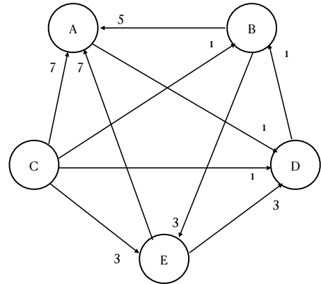
(b) V-IMDC-u counterexample
