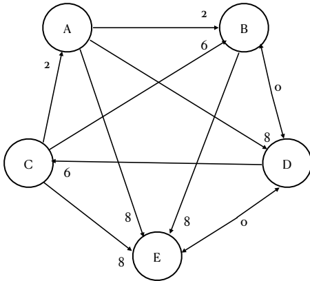
(a) P-IMDC-u counterexample
