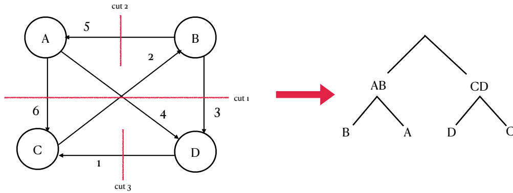
Fig. 1: An example of the IMDC procedure
